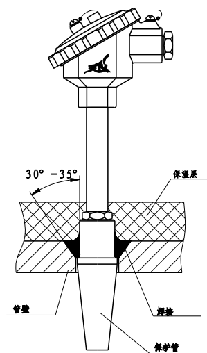
013T型安装示意 The installation sketching for type 013T
